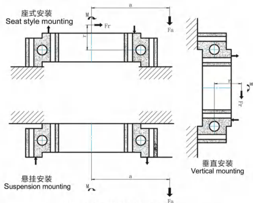
图2 回转支承安装形式示意图 Figure 2 Mounting sketch of slewing bearing
